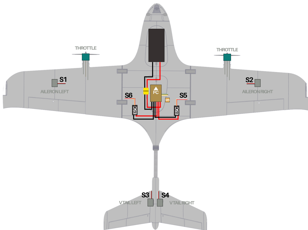
FLIGHTORY STALLION SAMPLE WIRING DIAGRAM
